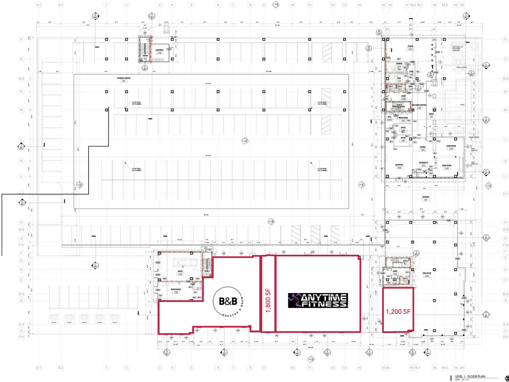
LEVEL 1 - FLOOR PLAN SCALE: 1/8" = 1'-0"
